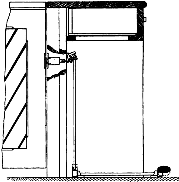
FIG. 27.—Treadle Latch for Open-Access Wicket (Section 160).
